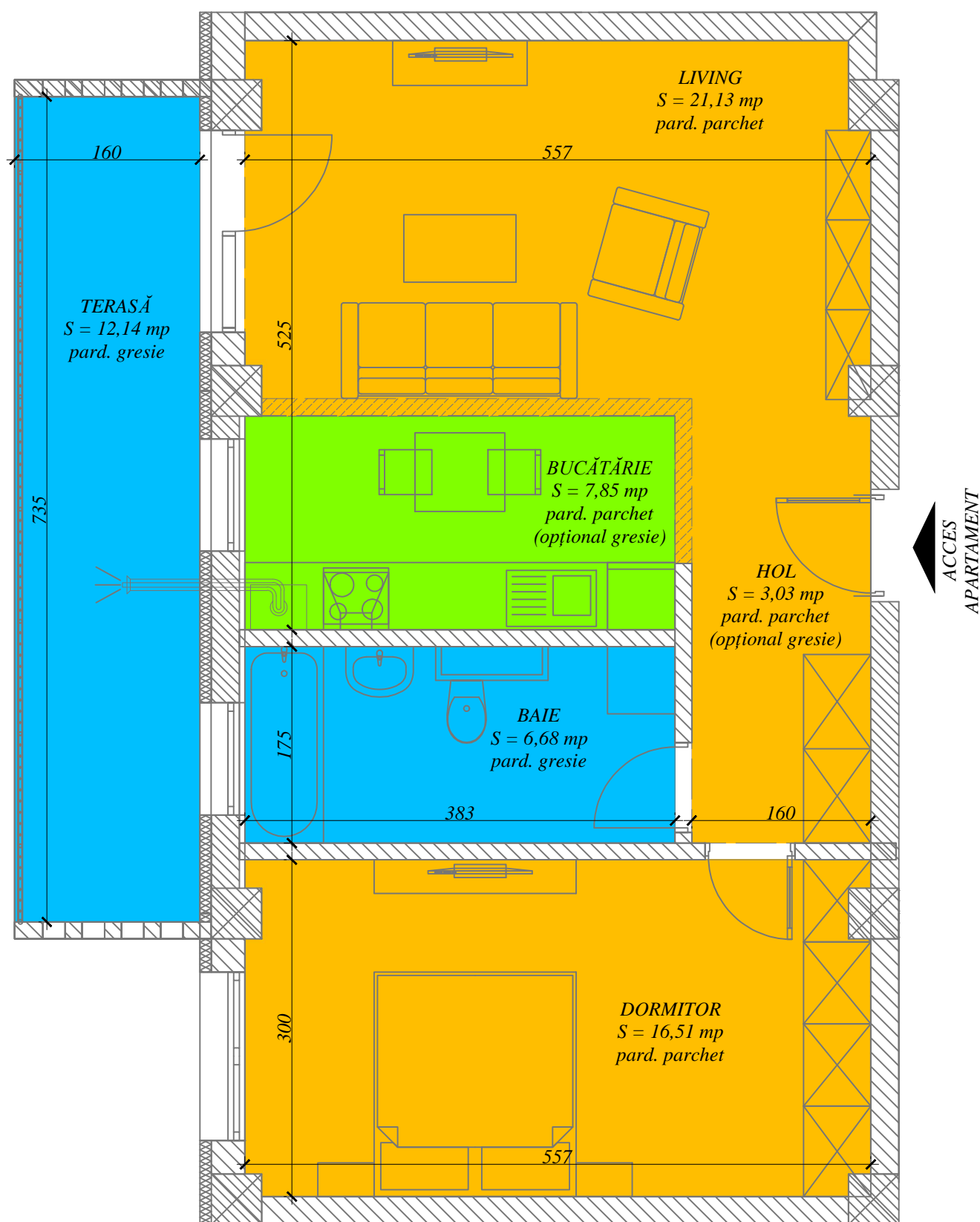
Plan AP. 33 imobil ELIZA 1, scara 1:50
