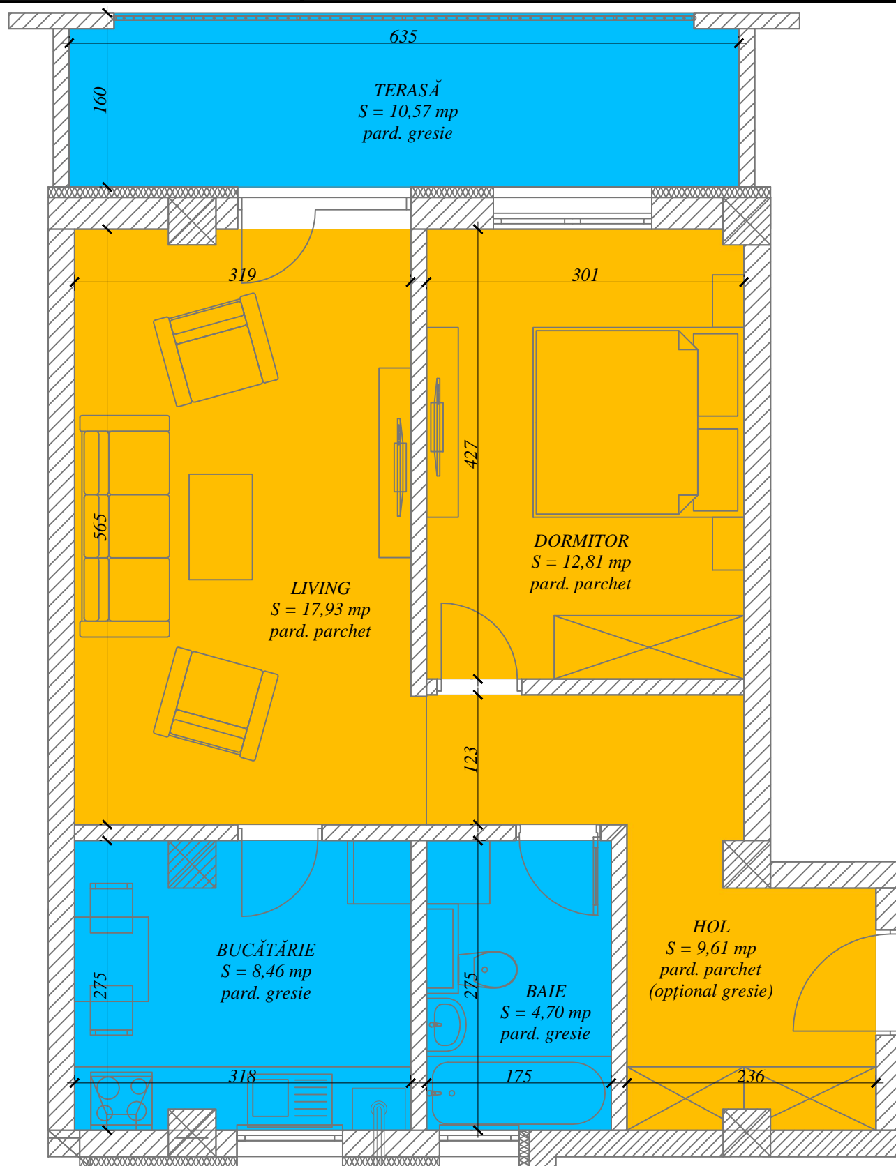
Plan AP. 29 imobil ELIZA 1, scara 1:50
