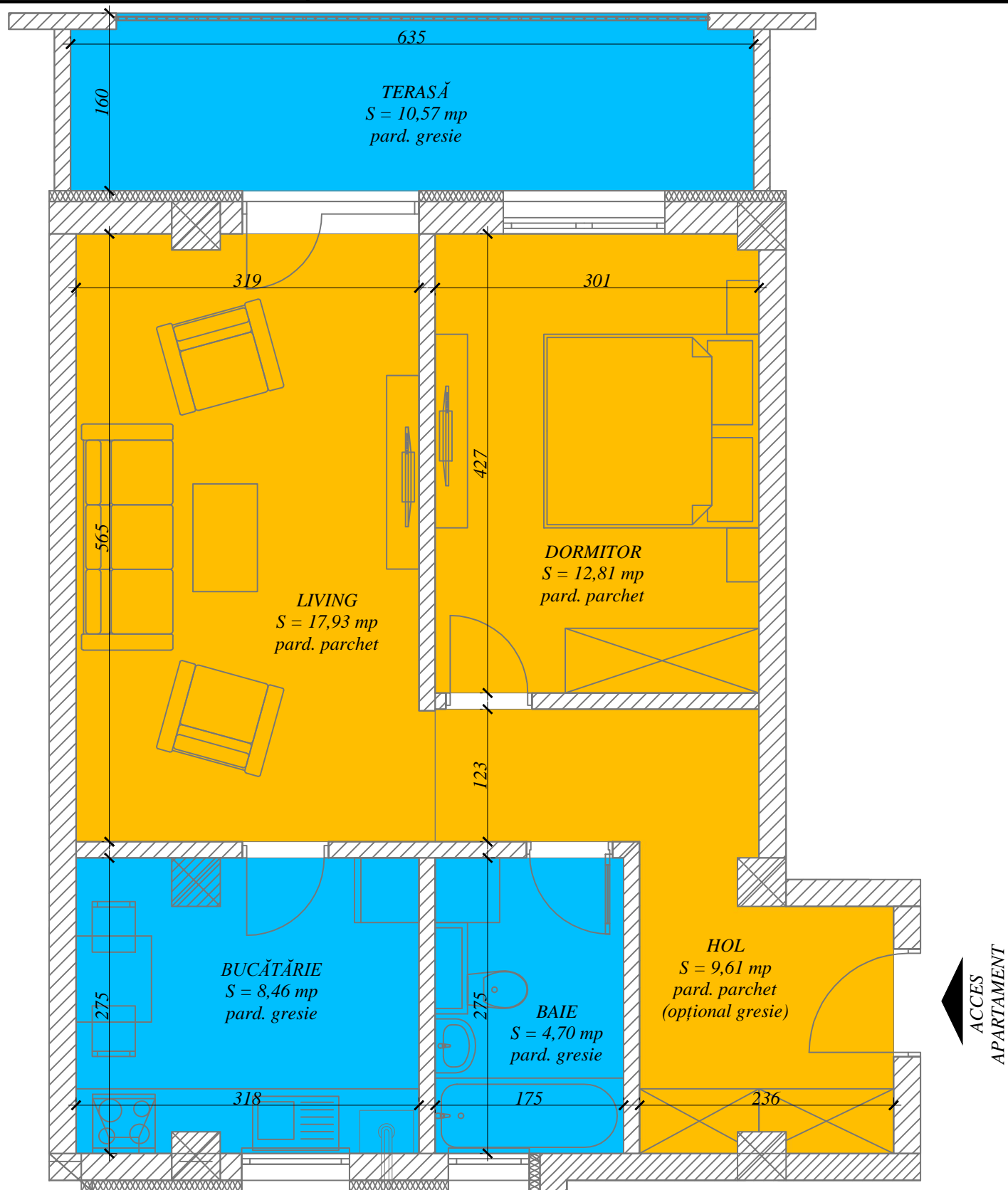
Plan AP. 18 imobil ELIZA 1, scara 1:50
