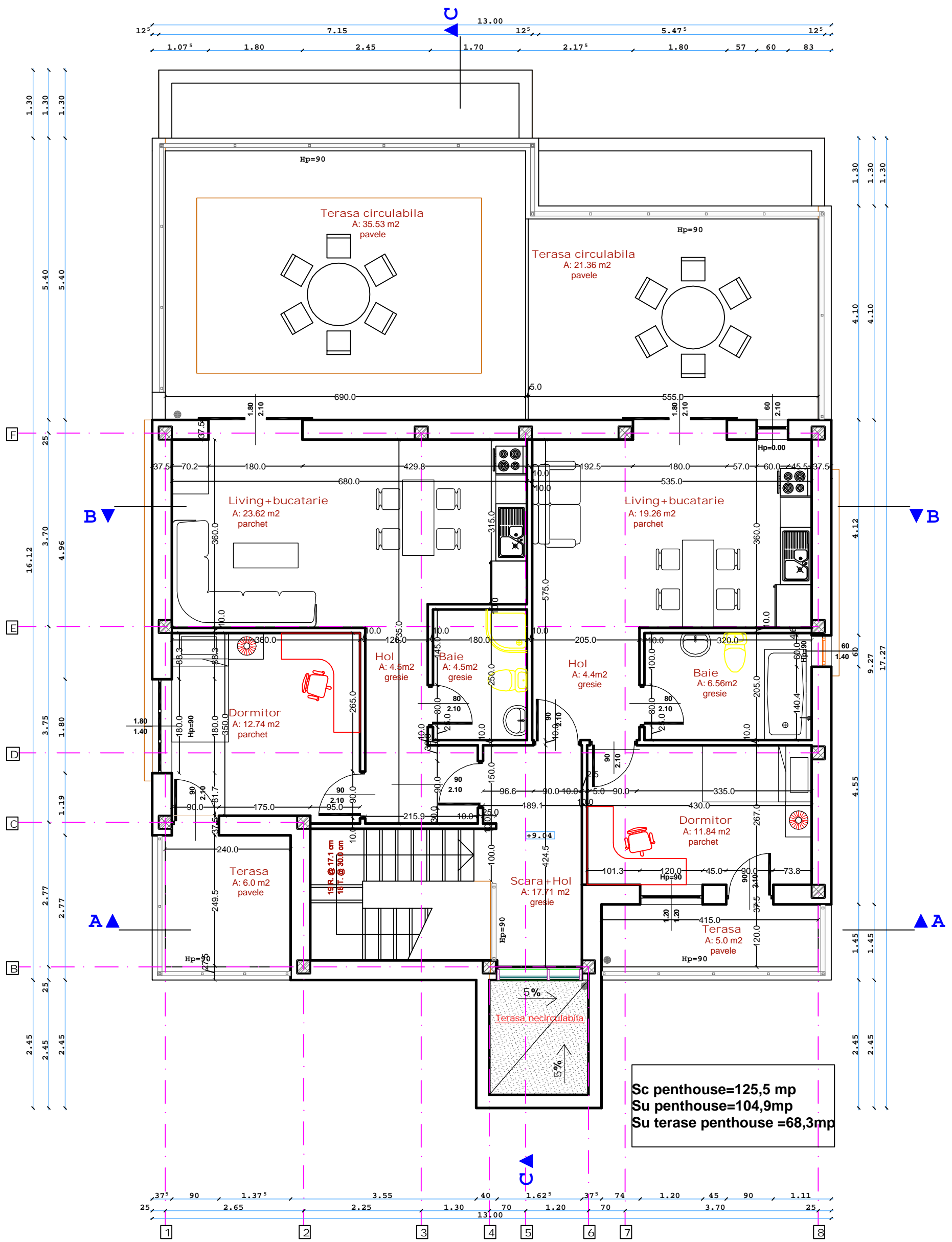
Plan penthouse sc. 1:50
